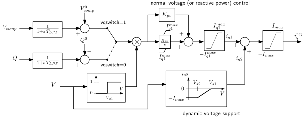
Figure 23.8: GFUL voltage/reactive power control and dynamic voltage support block diagram
