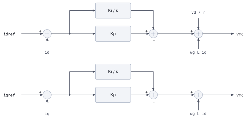
Figure 23.9: Grid-following inner current control.
