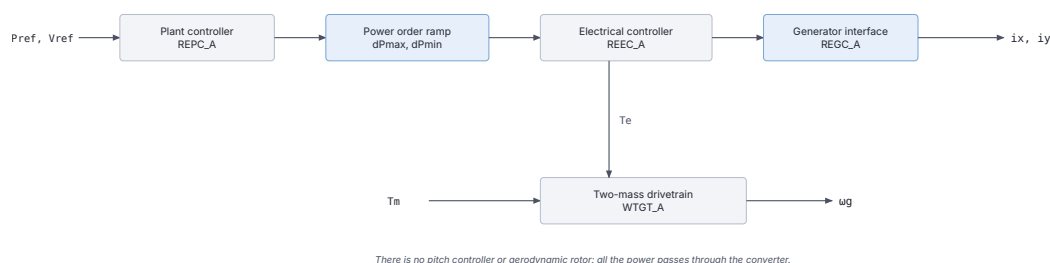
Figure 23.4: WT4 block diagram.
