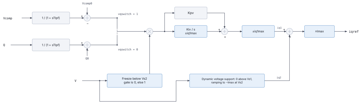
Figure 23.11: Grid-following voltage and reactive power control.
