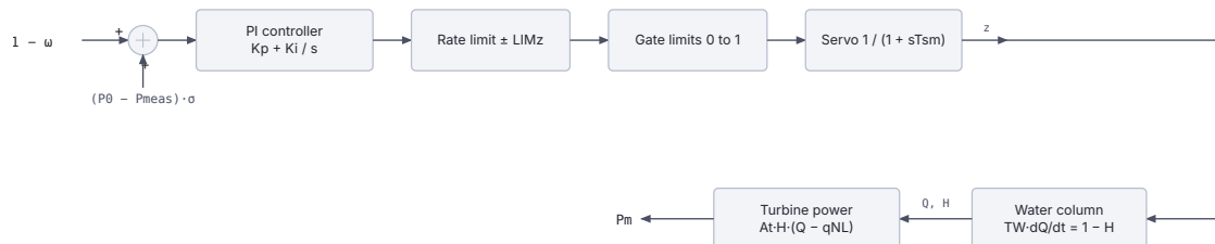
Figure 22.3: HYDRO_GENERIC1 block diagram.
