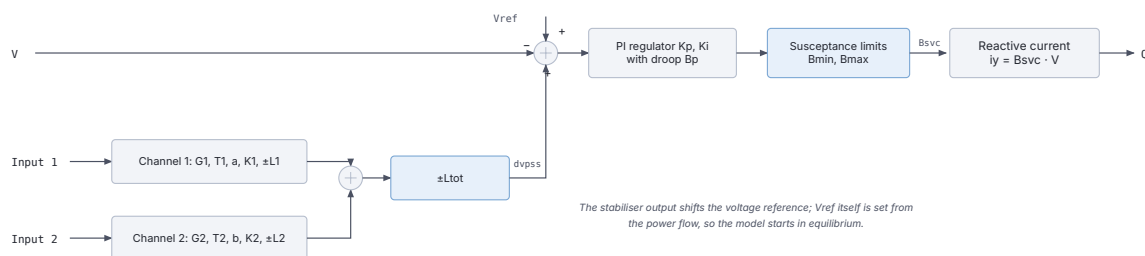
Figure 23.13: Generic static var compensator block diagram.
