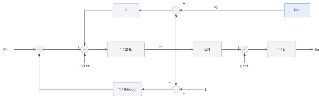
Figure 23.6: Grid-forming virtual synchronous machine block diagram.
