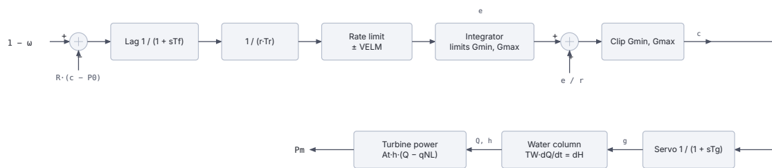
Figure 21.5: HYG0V block diagram.
