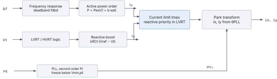
Figure 23.2: Generic inverter-based generator block diagram.
