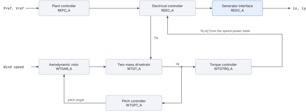
Figure 23.3: WT3 block diagram.
