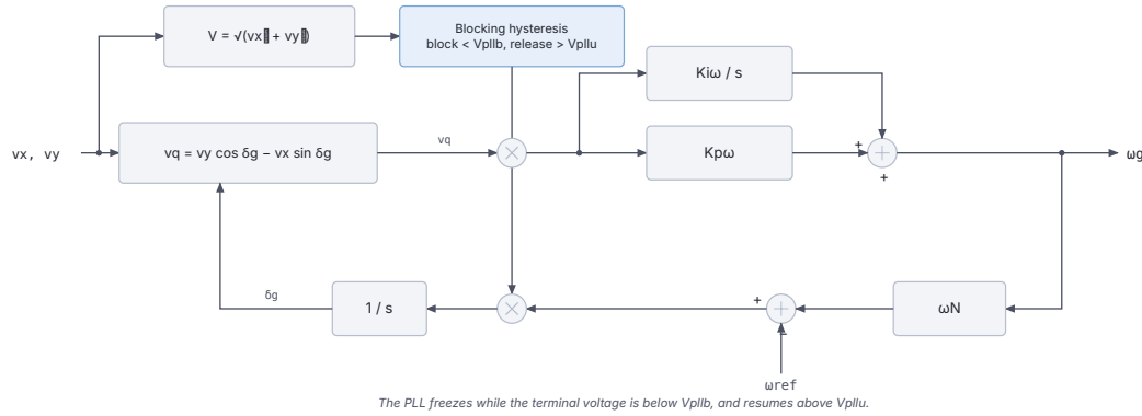
Figure 23.8: Grid-following phase-locked loop block diagram.
