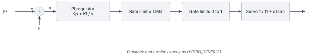
Figure 22.4: HYDRO_DG block diagram.
