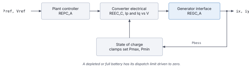
Figure 23.12: Battery energy storage block diagram.
