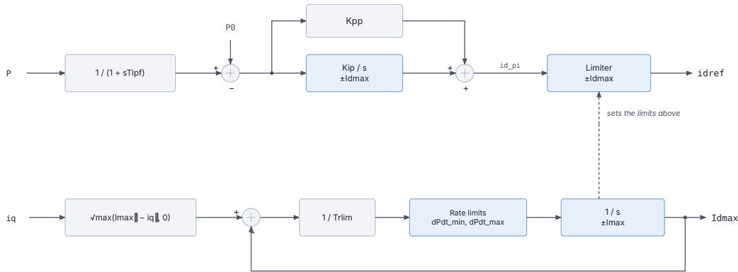
Figure 23.10: Grid-following active power control.
