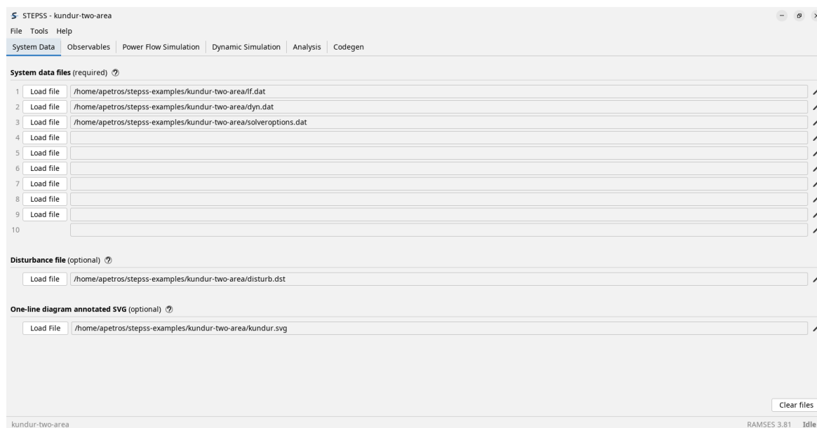
Figure 7.1: The System Data tab with the Kundur two-area case loaded.
