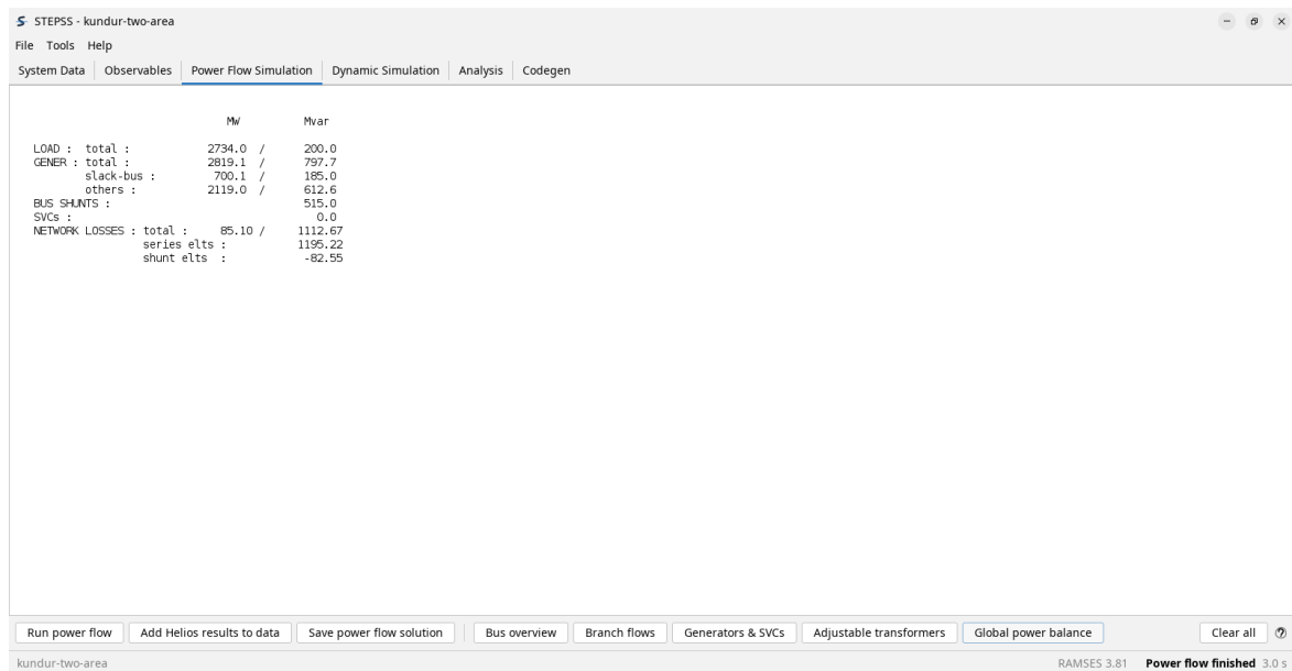
Figure 7.8: The Power Flow Simulation pane showing the global power balance for the Kundur case, in MW and Mvar.
