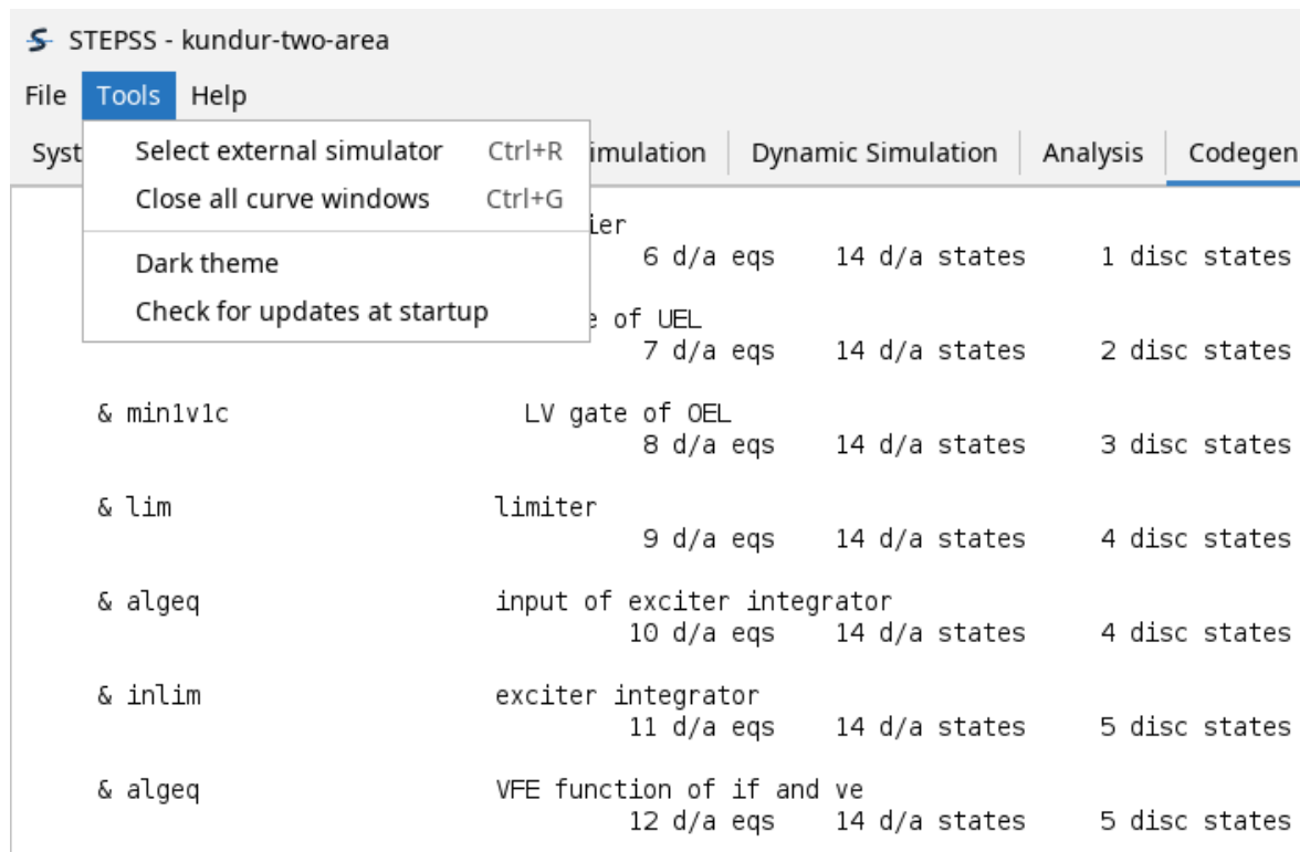
Figure 7.14: The Tools menu open, holding Select external simulator with Ctrl+R and Close all curve windows with Ctrl+G, then below a separator the Dark theme and Check for updates at startup ticks, both unticked.
