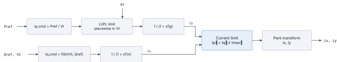
Figure 23.11: Photovoltaic generator block diagram.
