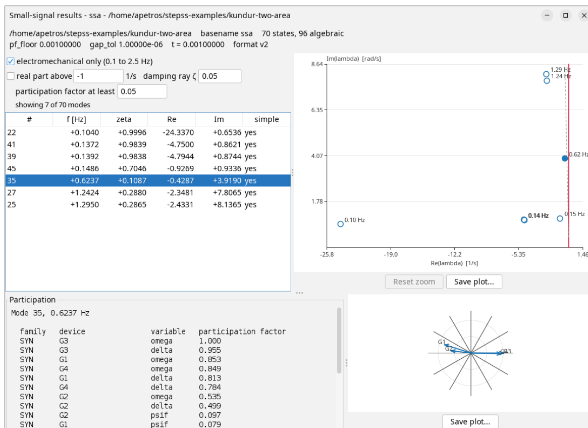
Figure 15.1: The small-signal results window for the Kundur case.
