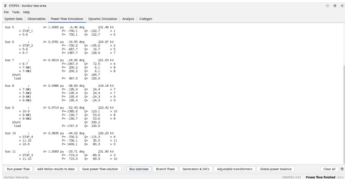
Figure 7.5: The Power Flow Simulation pane showing the bus overview for the Kundur case.
