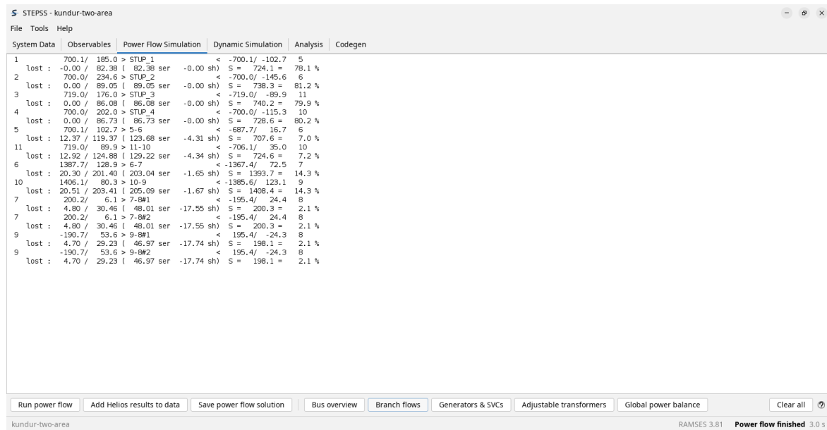
Figure 7.6: The Power Flow Simulation pane showing branch flows for the Kundur case.
