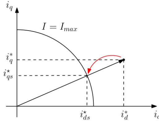
Figure 23.4: GFOR current limitation: proportional scaling of the dq current vector back to the I_{\max} circle and the modulated voltage is set to the value that yields the saturated currents:
