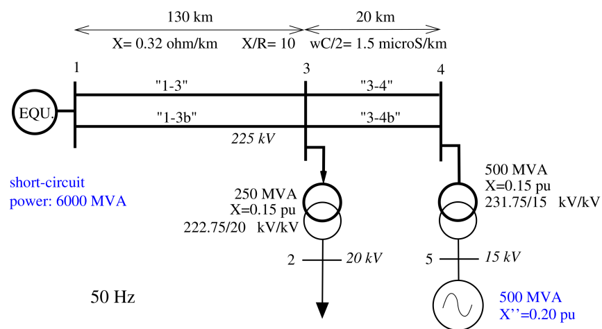
Figure 36.1: One-line diagram of the 5-bus test system
