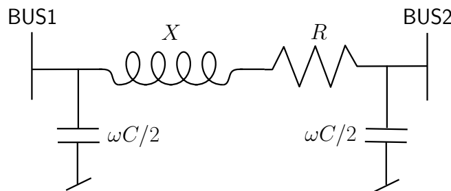
Figure 5.1: Pi-equivalent of lines and cables
