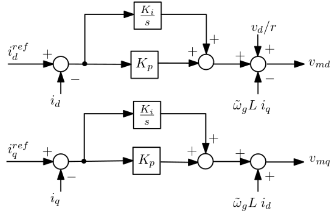
Figure 23.6: GFOL dq current control loops block diagram
