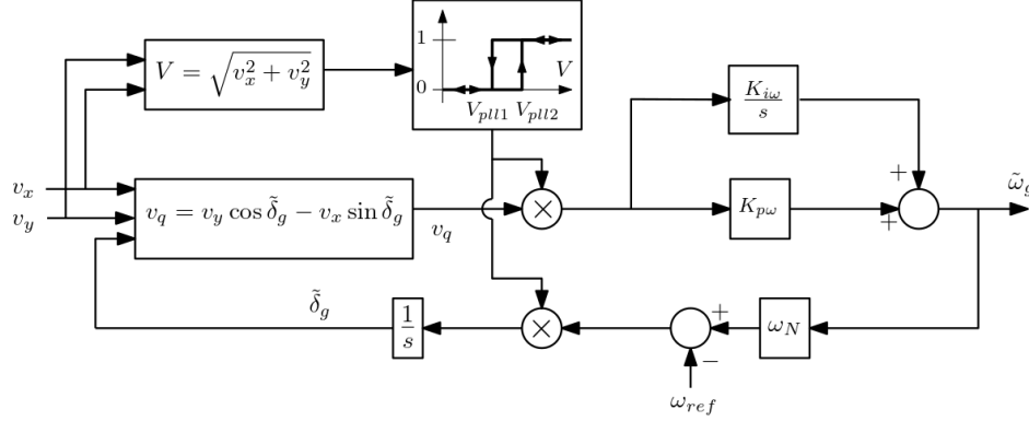
Figure 23.5: GFOF phase locked loop block diagram with blocking hysteresis
