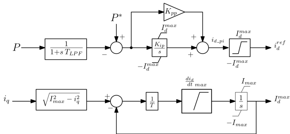
Figure 23.7: GFOL active power control and rate-limited d-axis current limit block diagram
