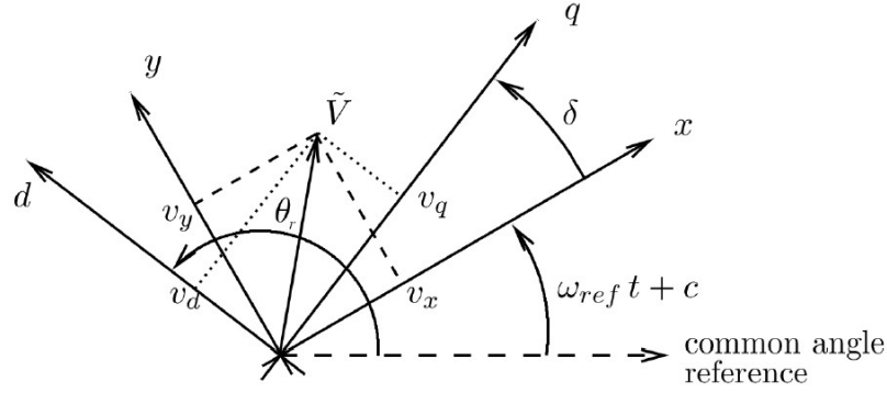
Figure 17.3: Definition of the rotor angle delta
