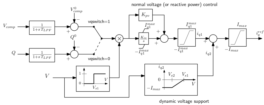
Figure 23.8: GFOL voltage/reactive power control and dynamic voltage support block diagram
