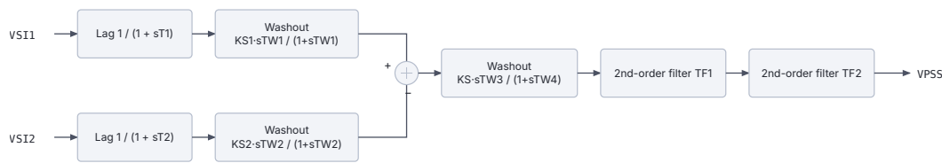
Figure 19.11: PSS3B block diagram.
