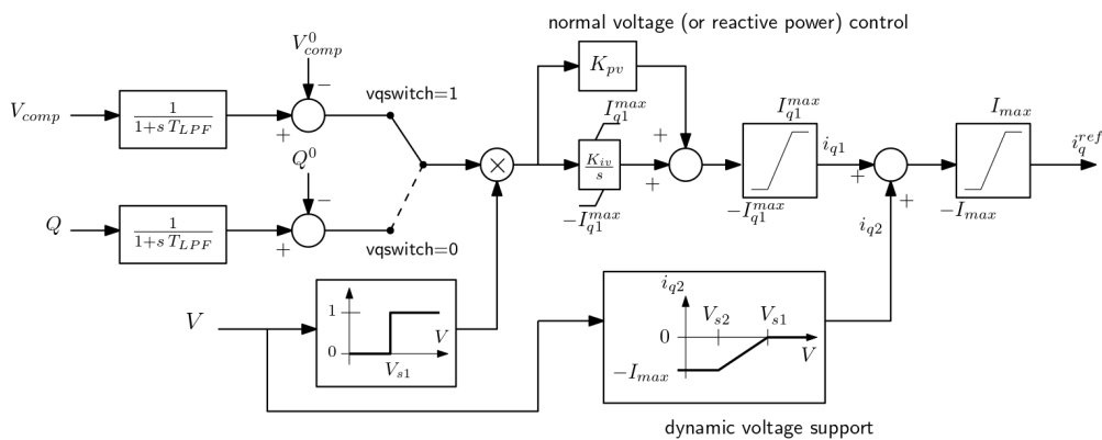
Figure 23.11: GFUL voltage/reactive power control and dynamic voltage support block diagram
