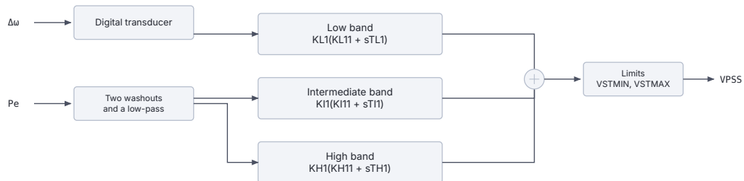
Figure 19.12: PSS4B block diagram.
