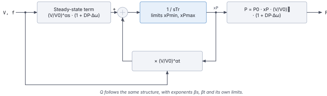
Figure 23.1: Exponential recovery load block diagram.
