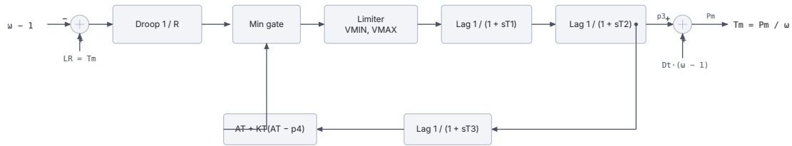
Figure 21.3: GAST block diagram.
