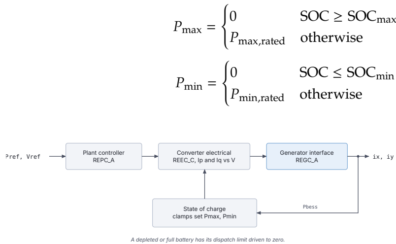
Figure 23.12: Battery energy storage block diagram.
