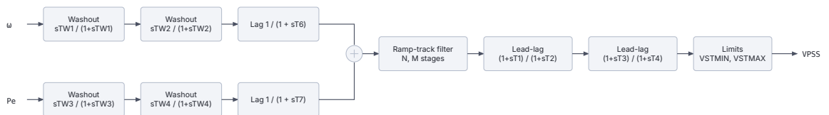
Figure 19.10: PSS2B block diagram.
