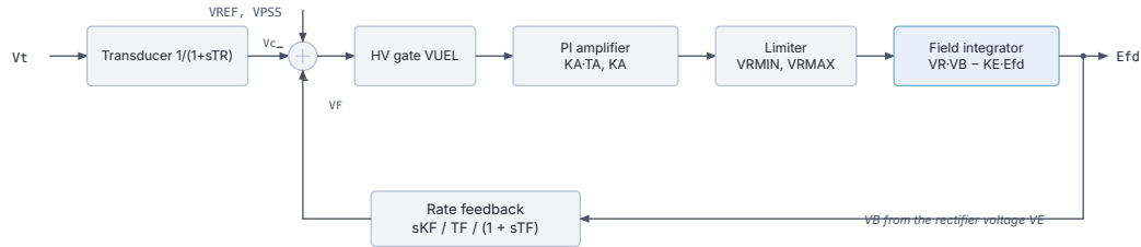
Figure 19.6: ST2A block diagram.
