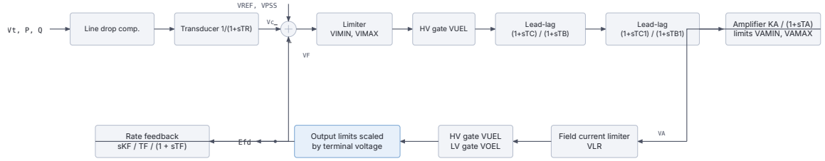
Figure 19.5: ST1A block diagram.
