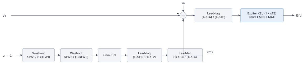
Figure 19.9: ENTSGE_simp block diagram.
