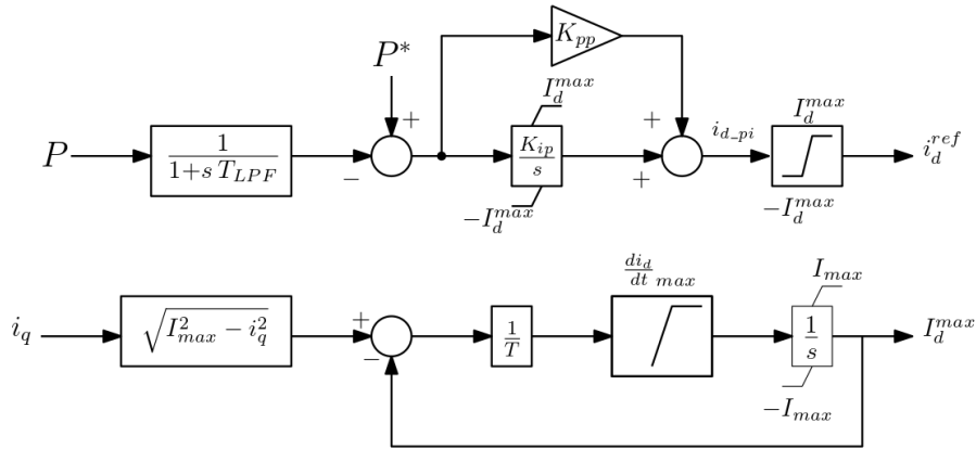
Figure 23.10: GFUL active power control and rate-limited d-axis current limit block diagram
