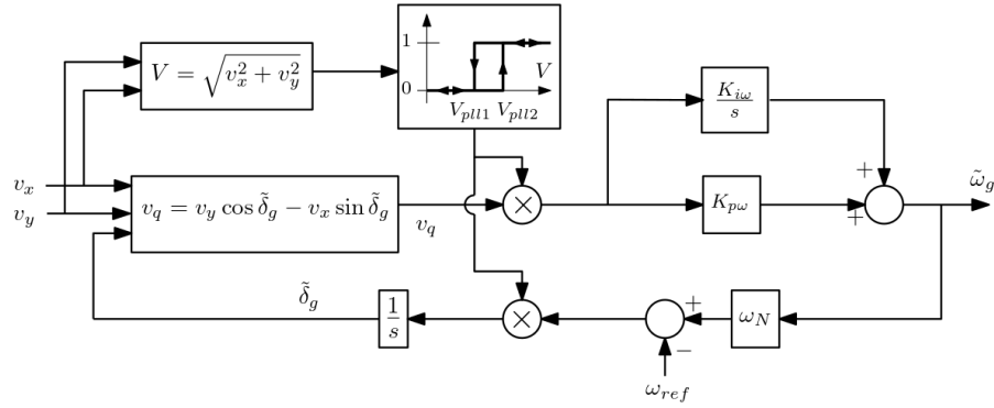
Figure 23.8: GFOL phase locked loop block diagram with blocking hysteresis
