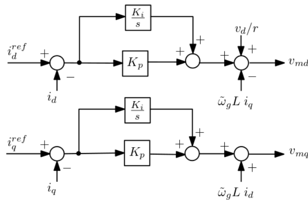
Figure 23.9: GFOL dq current control loops block diagram
