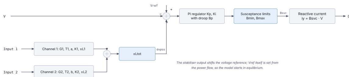
Figure 23.13: Generic static var compensator block diagram.
