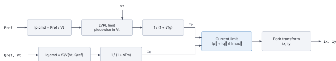
Figure 23.5: Photovoltaic generator block diagram.
