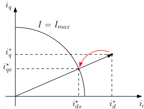
Figure 23.7: GFOR current limitation: proportional scaling of the dq current vector back to the I_{\max} circle
