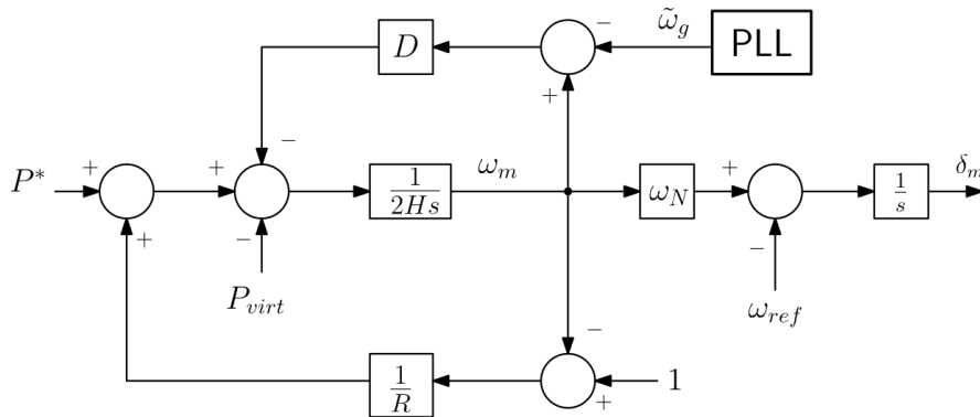
Figure 23.6: GFOR virtual synchronous machine active power and phase angle control block diagram
