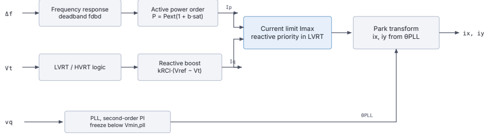
Figure 23.2: Generic inverter-based generator block diagram.
