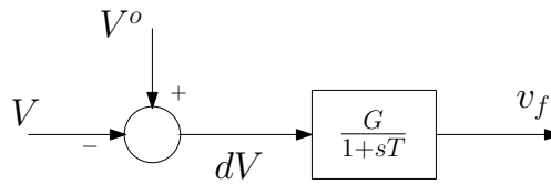
Figure 11.2: A very simple model of excitation system
