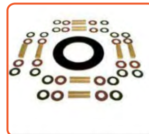
Type F (Raised Face Type Gasket)
