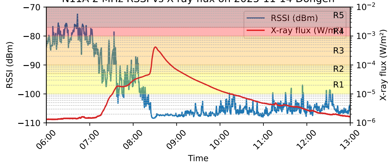
N11A 2 MHz RSSI vs X-ray flux on 2025-11-14 Dongen
