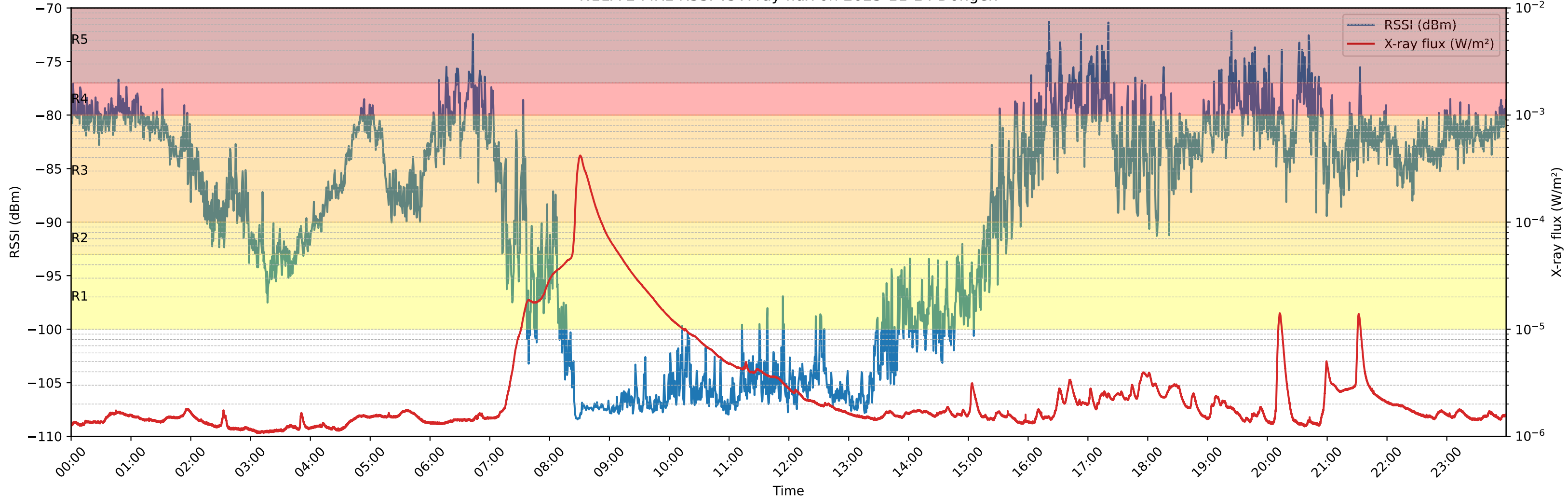
N11A 2 MHz RSSI vs X-ray flux on 2025-11-14 Dongen
