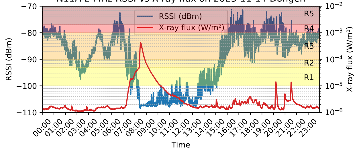
N11A 2 MHz RSSI vs X-ray flux on 2025-11-14 Dongen
