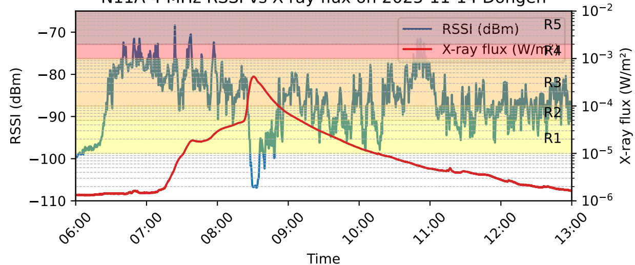
N11A 4 MHz RSSI vs X-ray flux on 2025-11-14 Dongen
