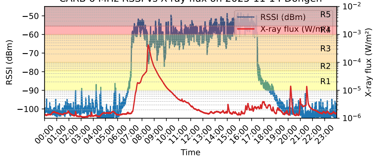
CARB 6 MHz RSSI vs X-ray flux on 2025-11-14 Dongen
