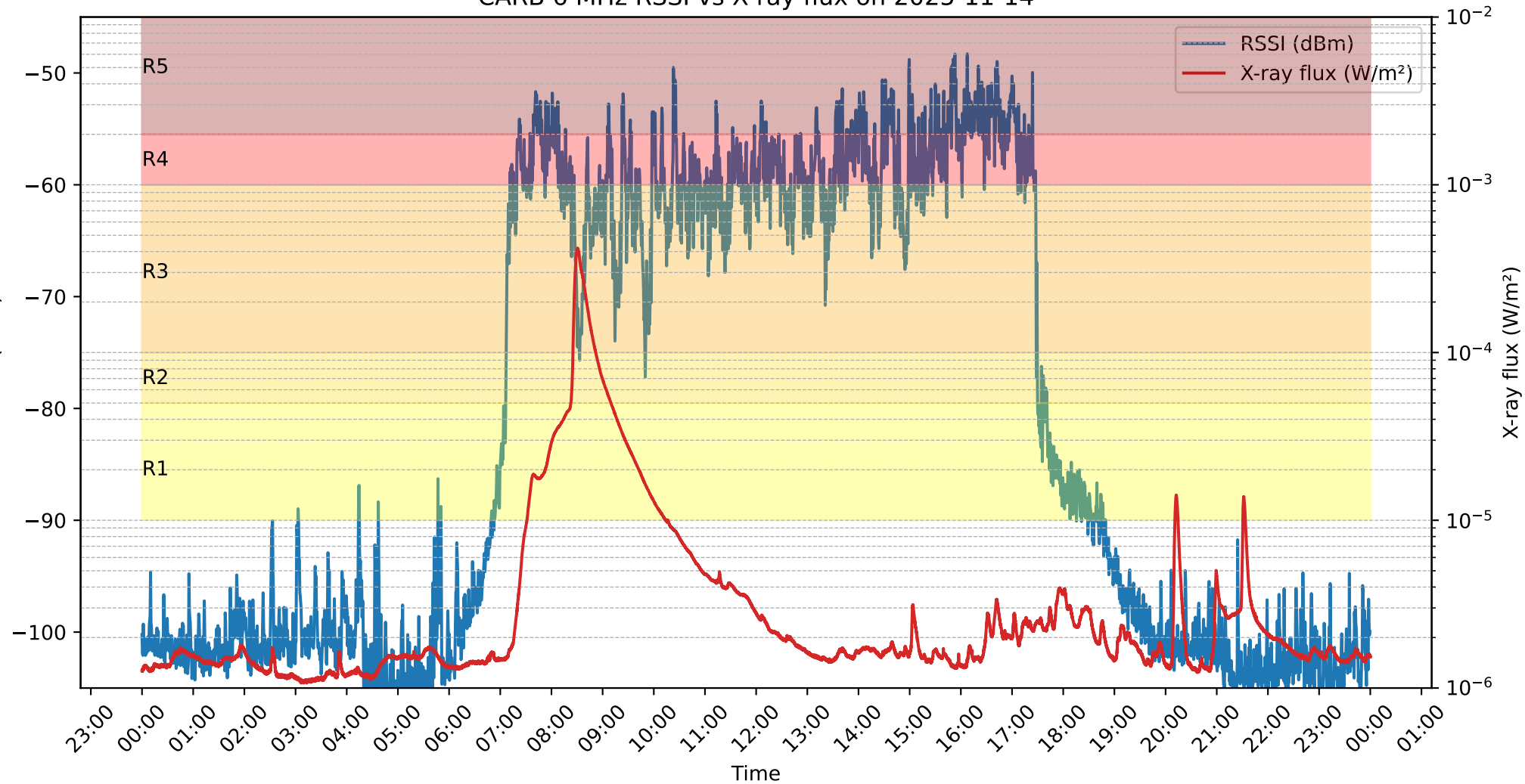
CARB 6 MHz RSSI vs X-ray flux on 2025-11-14
