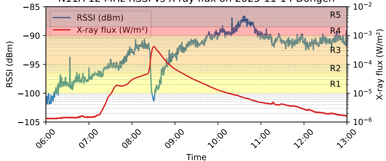
N11A 12 MHz RSSI vs X-ray flux on 2025-11-14 Dongen
