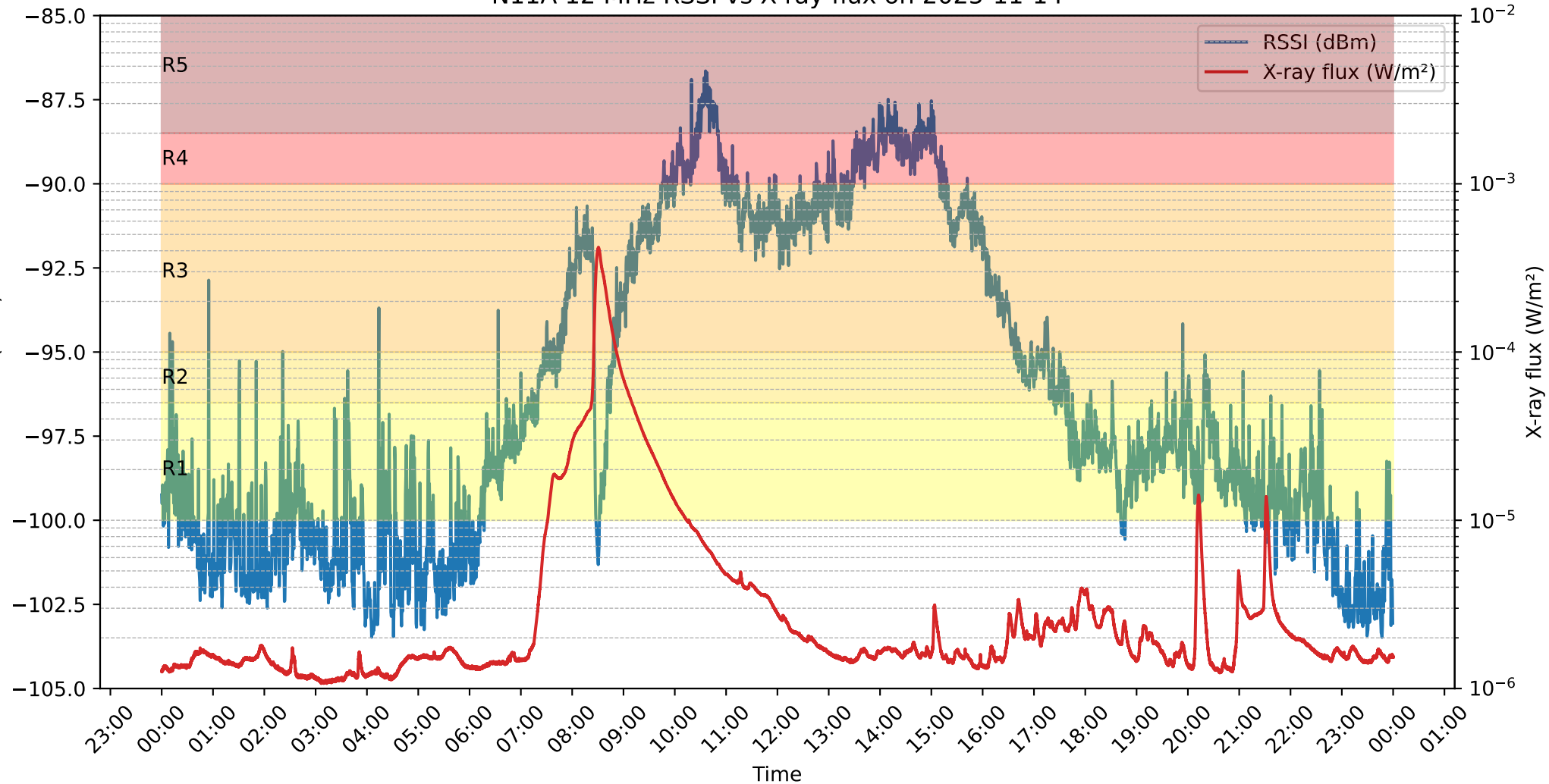
N11A 12 MHz RSSI vs X-ray flux on 2025-11-14
