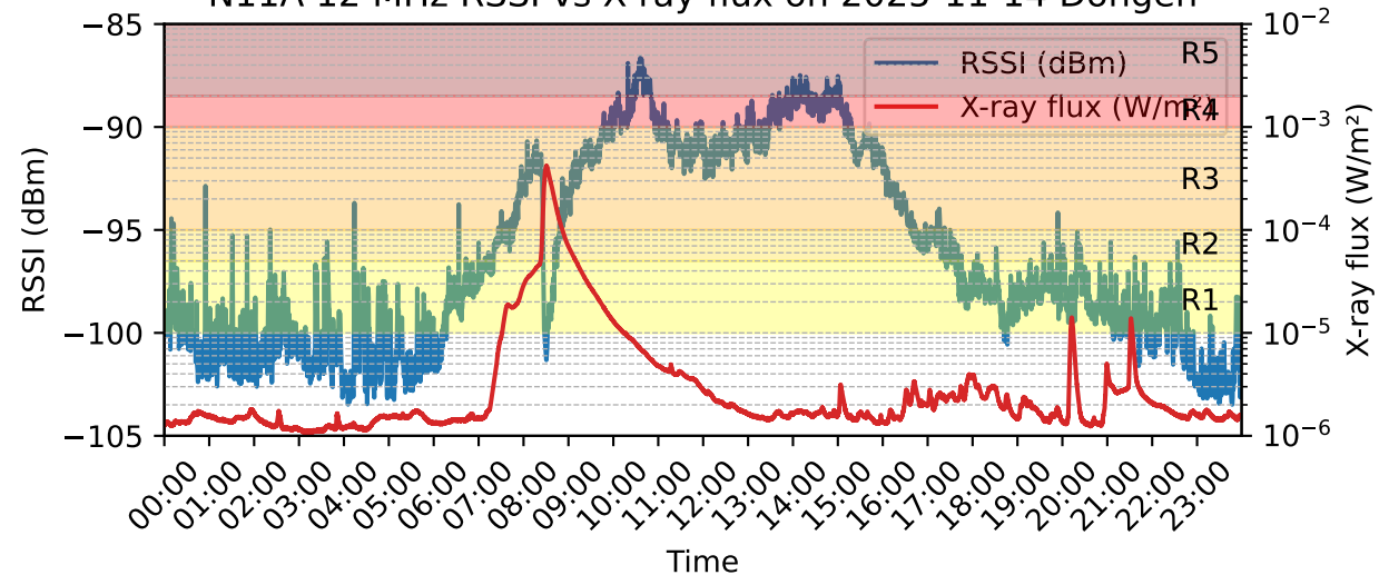
N11A 12 MHz RSSI vs X-ray flux on 2025-11-14 Dongen
