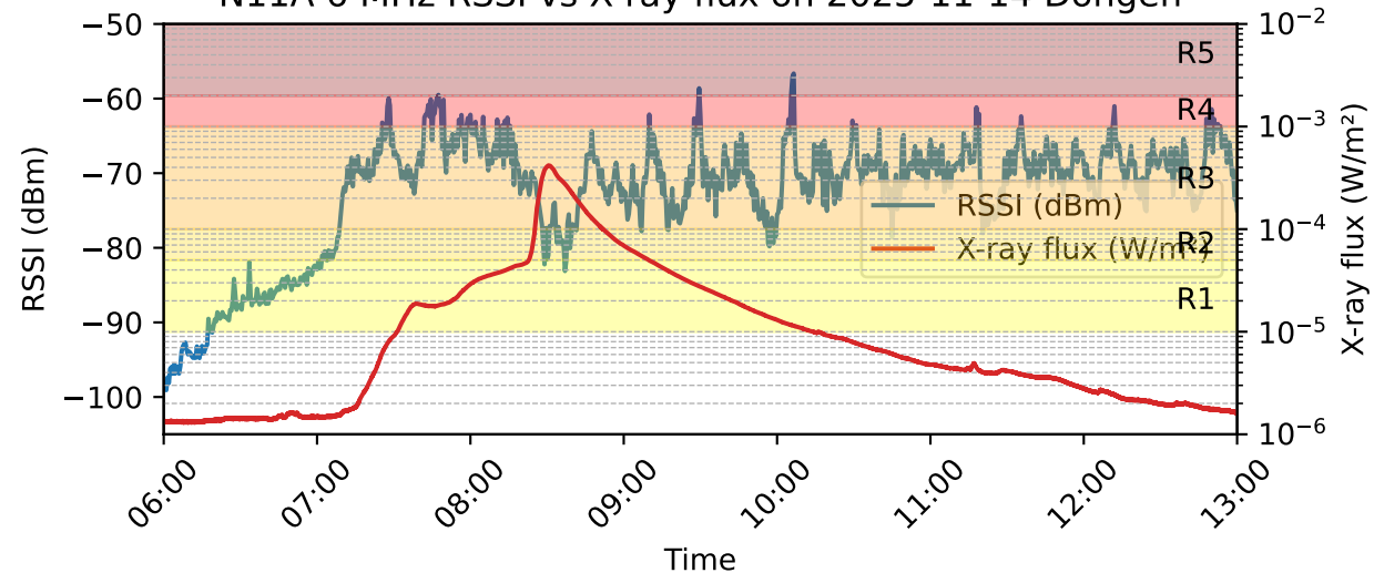
N11A 6 MHz RSSI vs X-ray flux on 2025-11-14 Dongen
