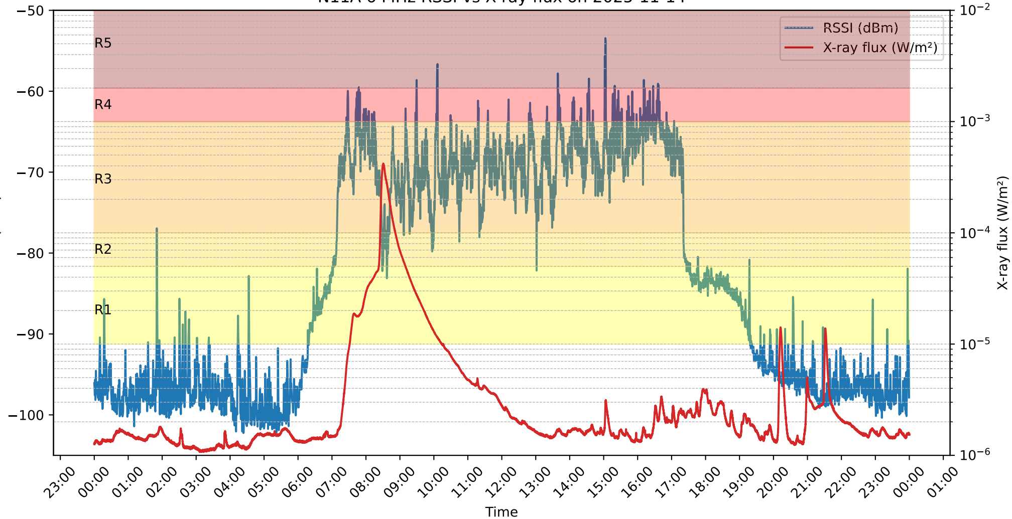
N11A 6 MHz RSSI vs X-ray flux on 2025-11-14
