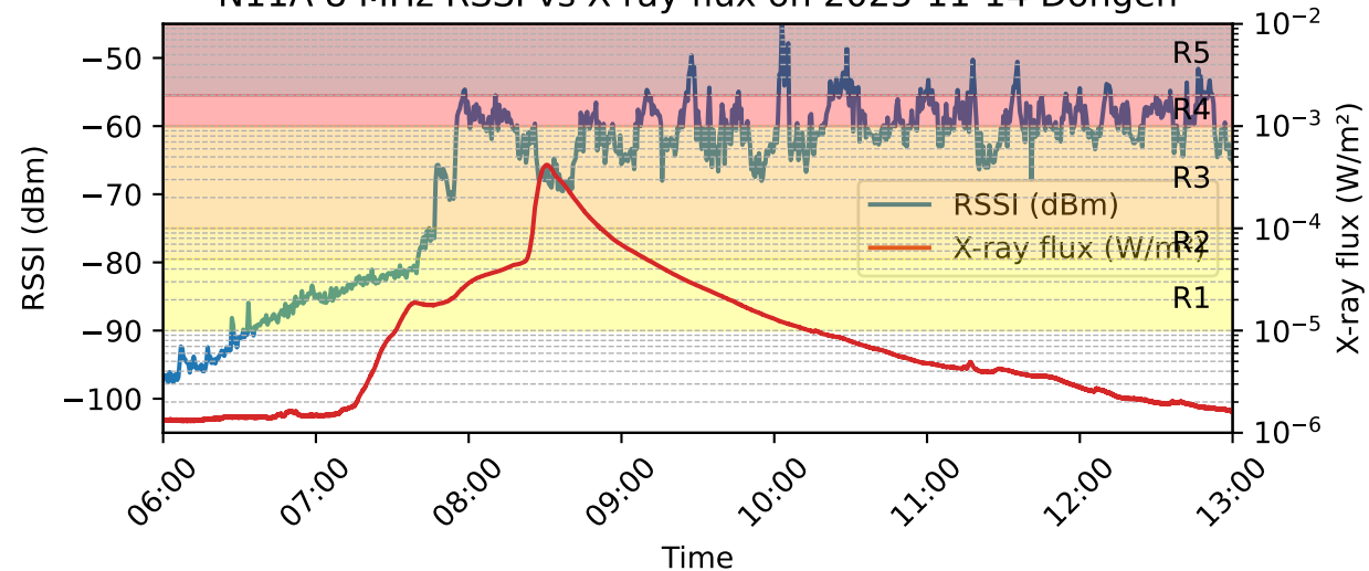
N11A 8 MHz RSSI vs X-ray flux on 2025-11-14 Dongen
