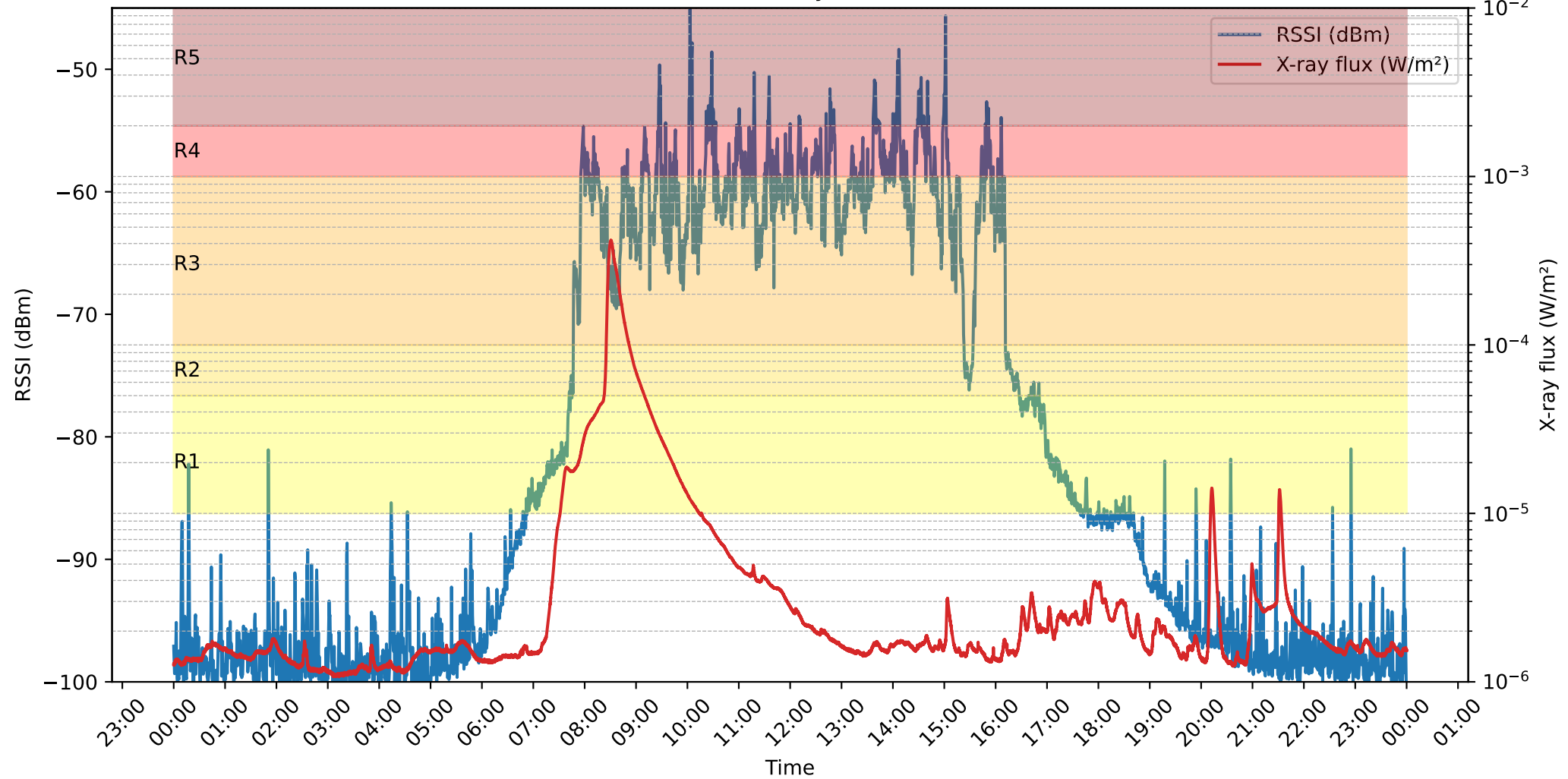
N11A 8 MHz RSSI vs X-ray flux on 2025-11-14
