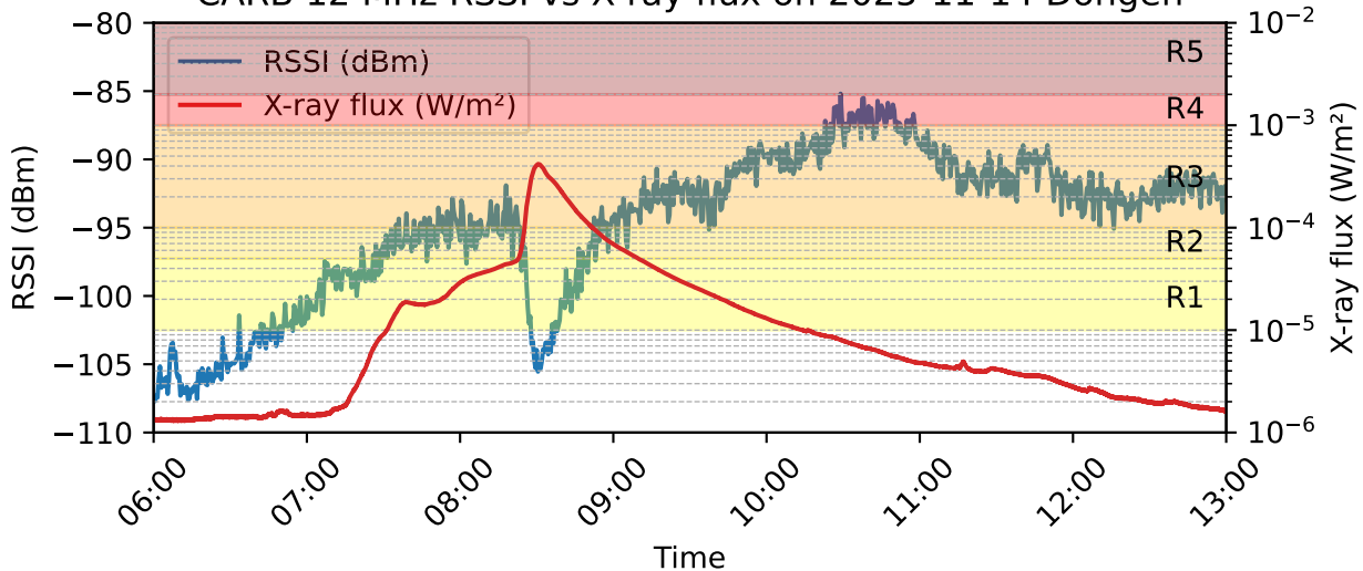
CARB 12 MHz RSSI vs X-ray flux on 2025-11-14 Dongen
