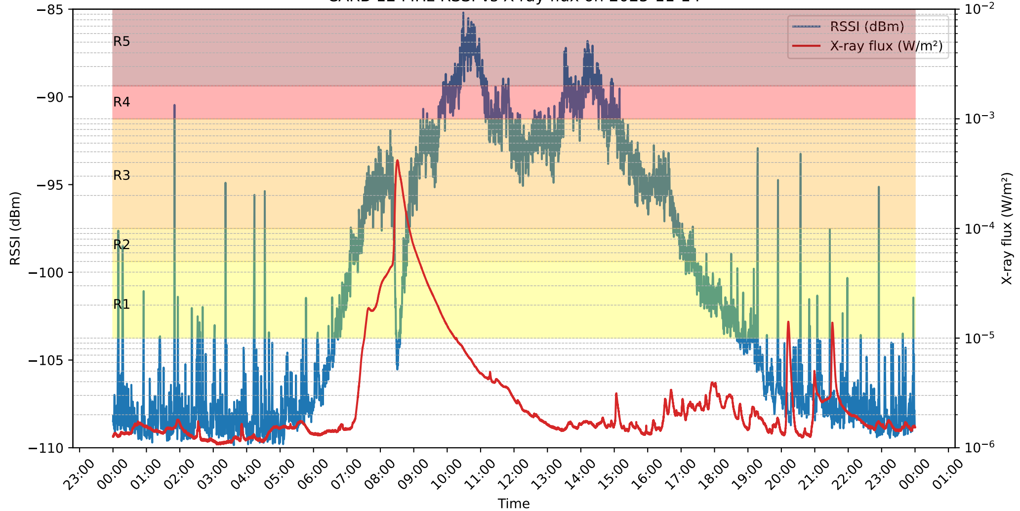
CARB 12 MHz RSSI vs X-ray flux on 2025-11-14
