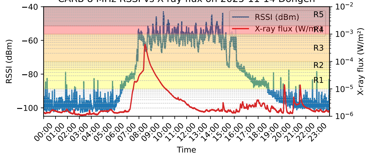
CARB 8 MHz RSSI vs X-ray flux on 2025-11-14 Dongen
