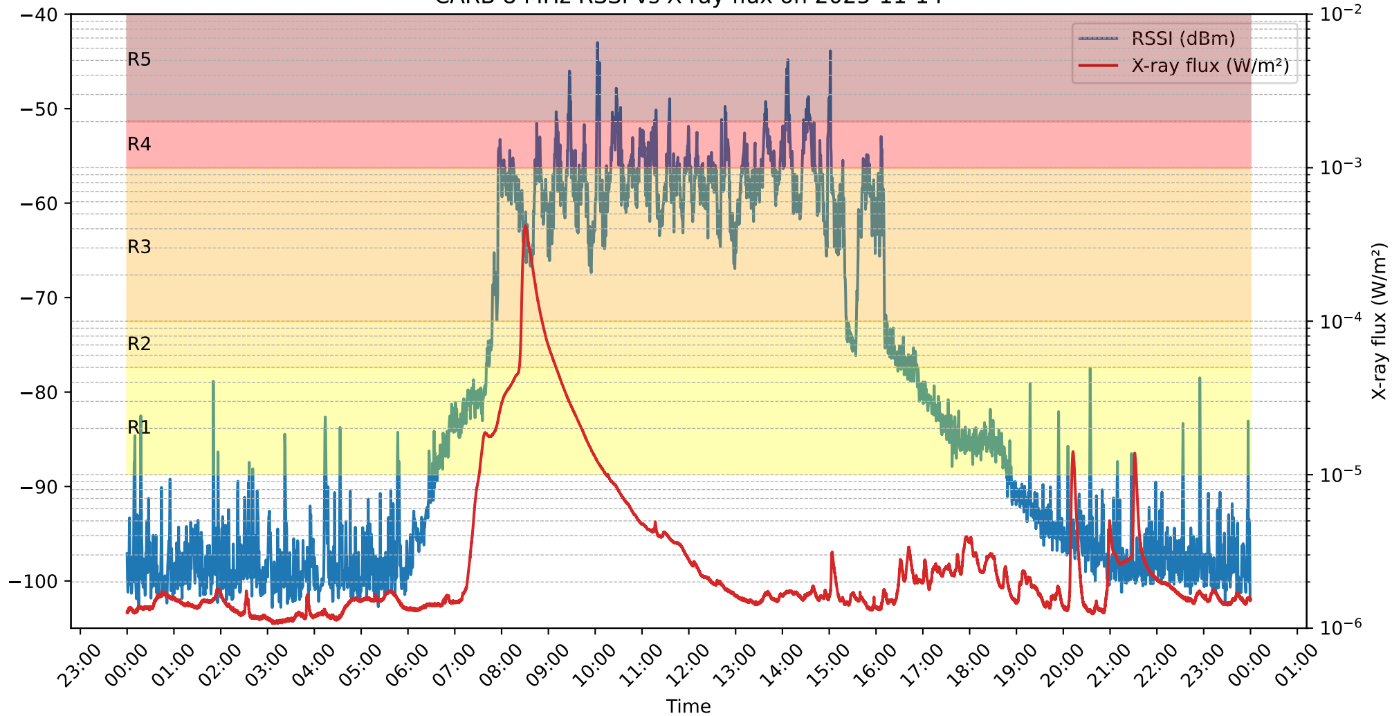
CARB 8 MHz RSSI vs X-ray flux on 2025-11-14
