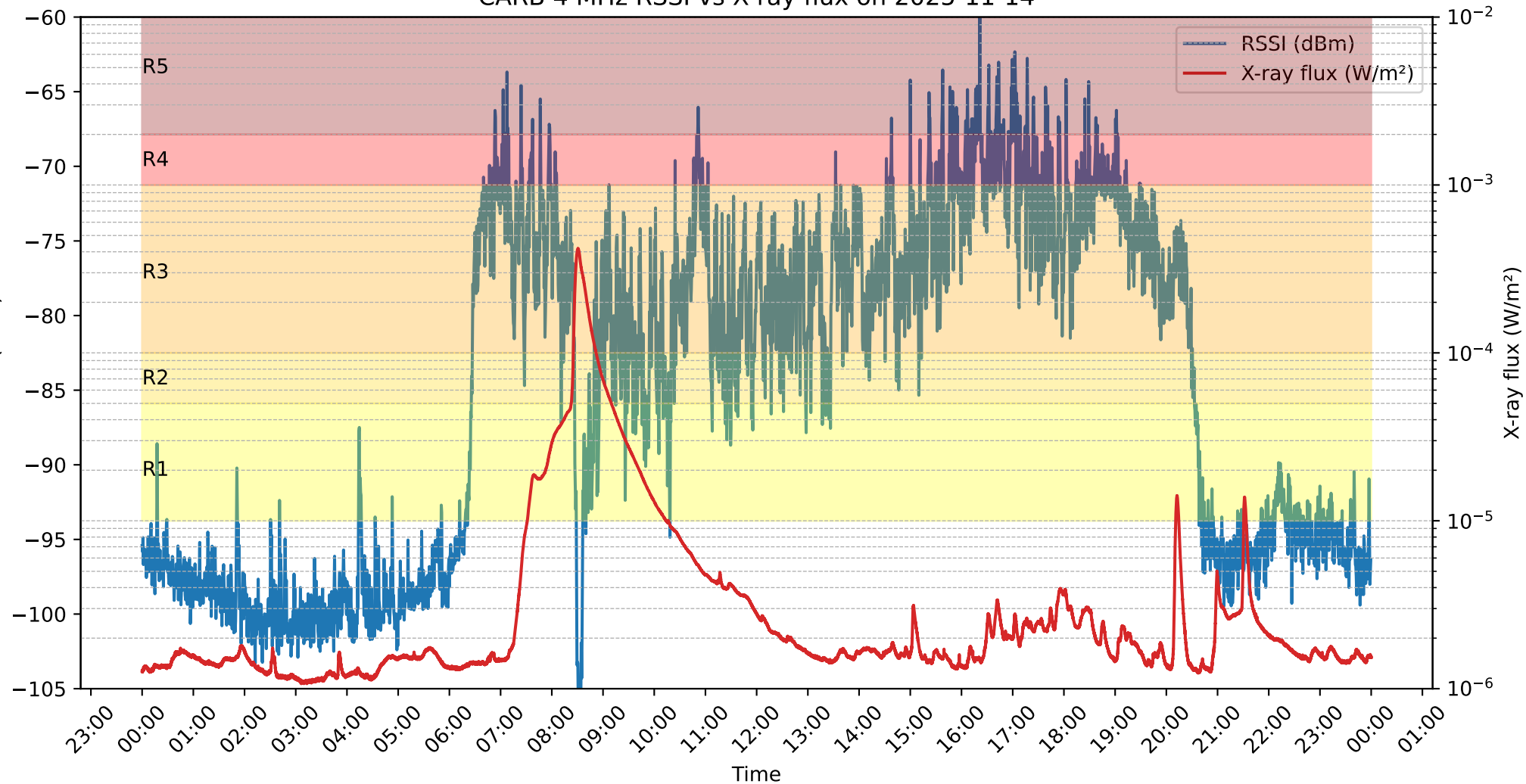
CARB 4 MHz RSSI vs X-ray flux on 2025-11-14
