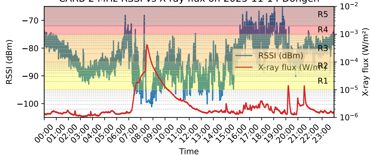
CARB 2 MHz RSSI vs X-ray flux on 2025-11-14 Dongen
