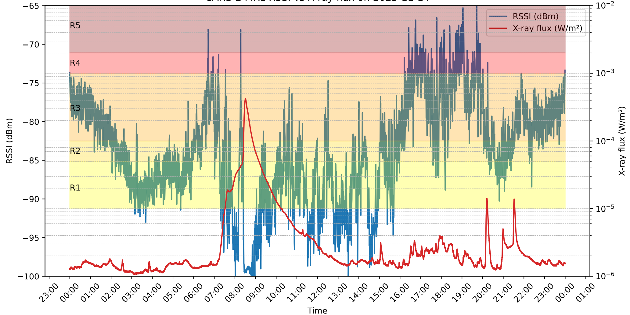
CARB 2 MHz RSSI vs X-ray flux on 2025-11-14
