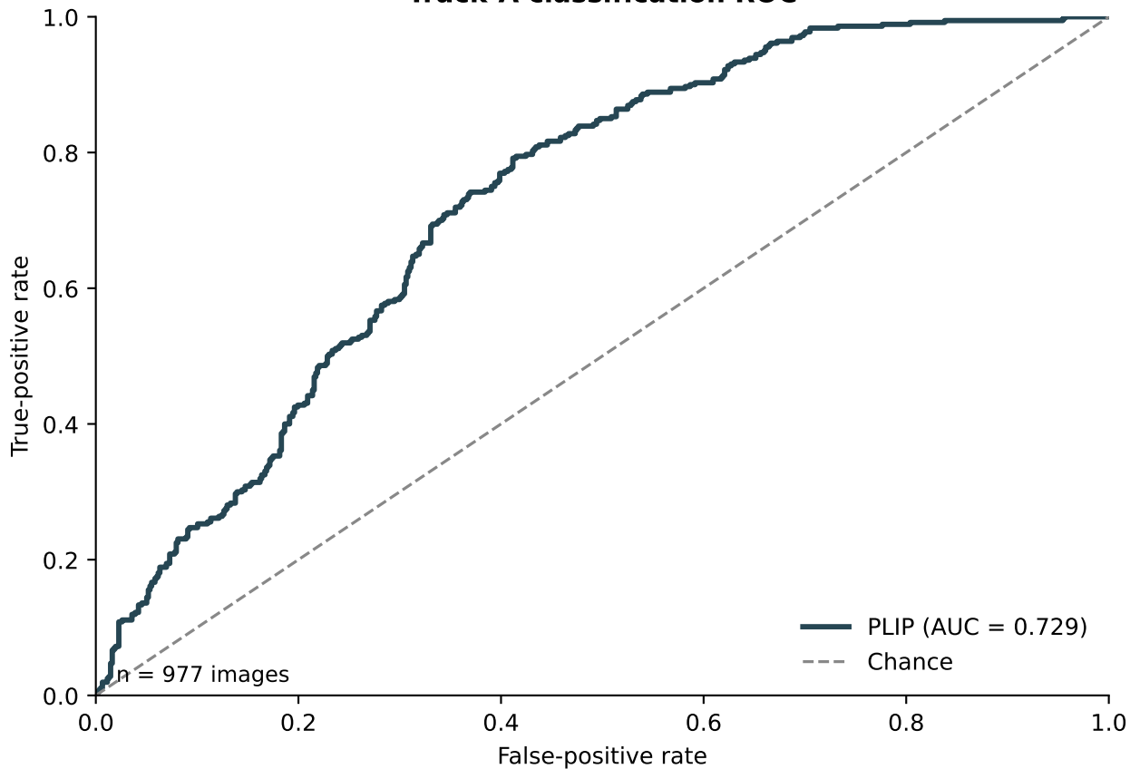
Track-A classification ROC
