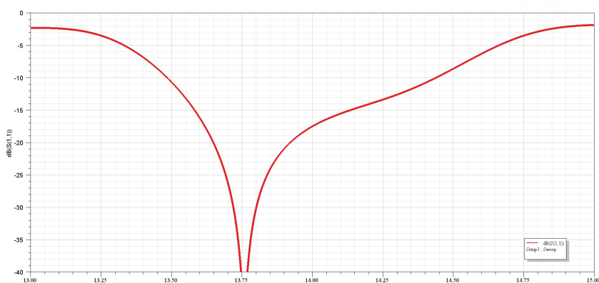
Figure 5: |S_{11}| (dB) vs frequency for the 1 \times 8 element array. The resonance occurs near 13.75 GHz with |S_{11}| < -40 dB. 🚀
