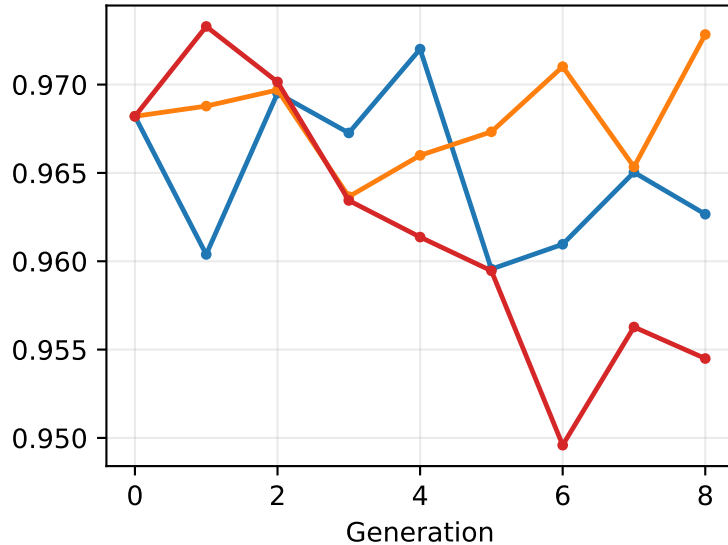
Canonical share
