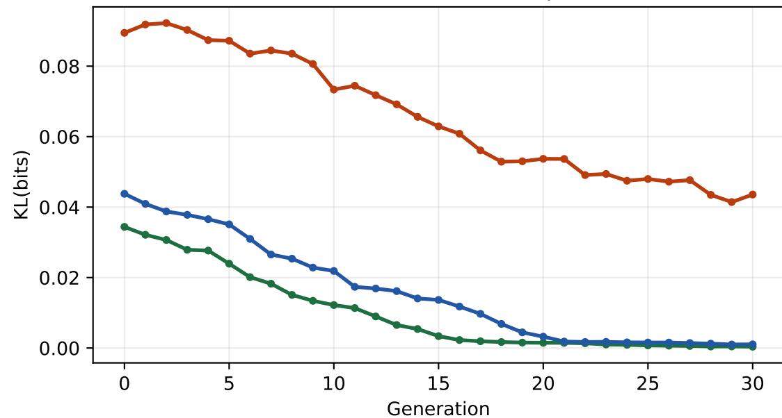
Exact KL(bits) to one-step law
