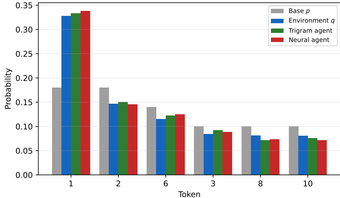
Representative context c=(2 \ 1) at 50k pairs
