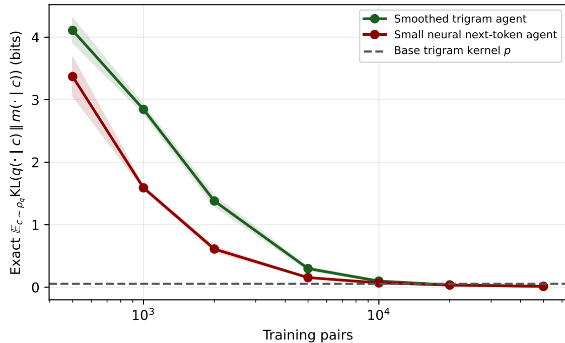
Both agent classes approach the same evolved environment q
