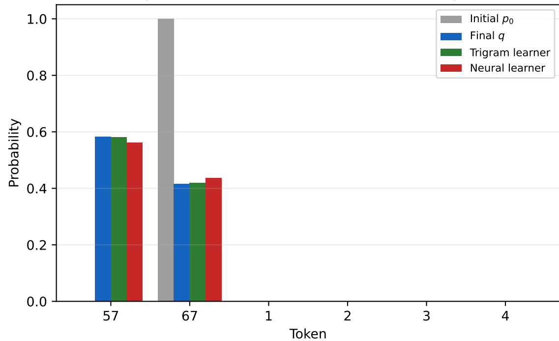
Representative context c=(80\ 55) at 20k pairs
