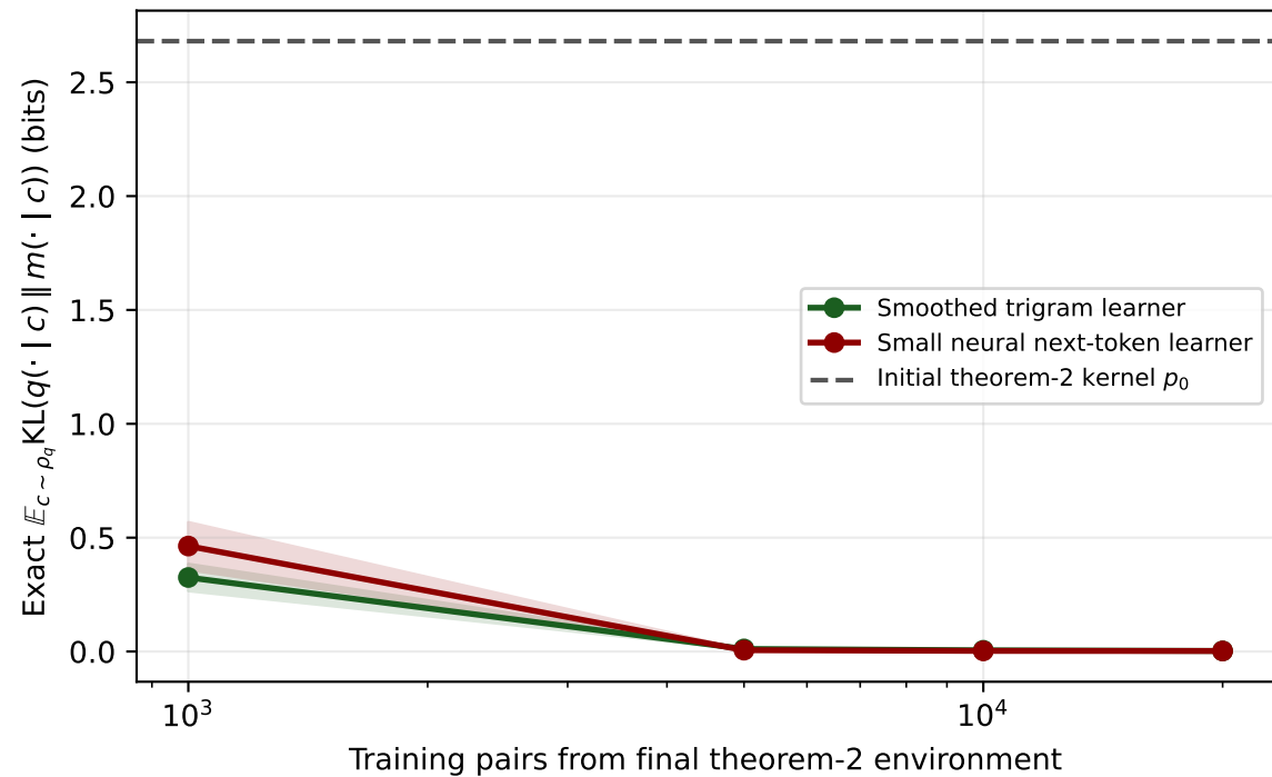
Downstream learners recover the final theorem-2 environment
