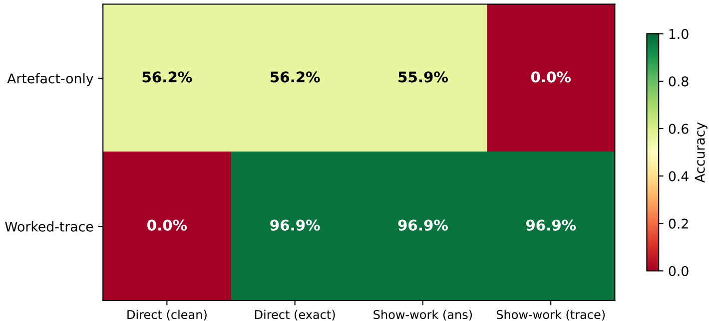
Environment x deployment mode interaction (same problems, same architecture, different text environments)
