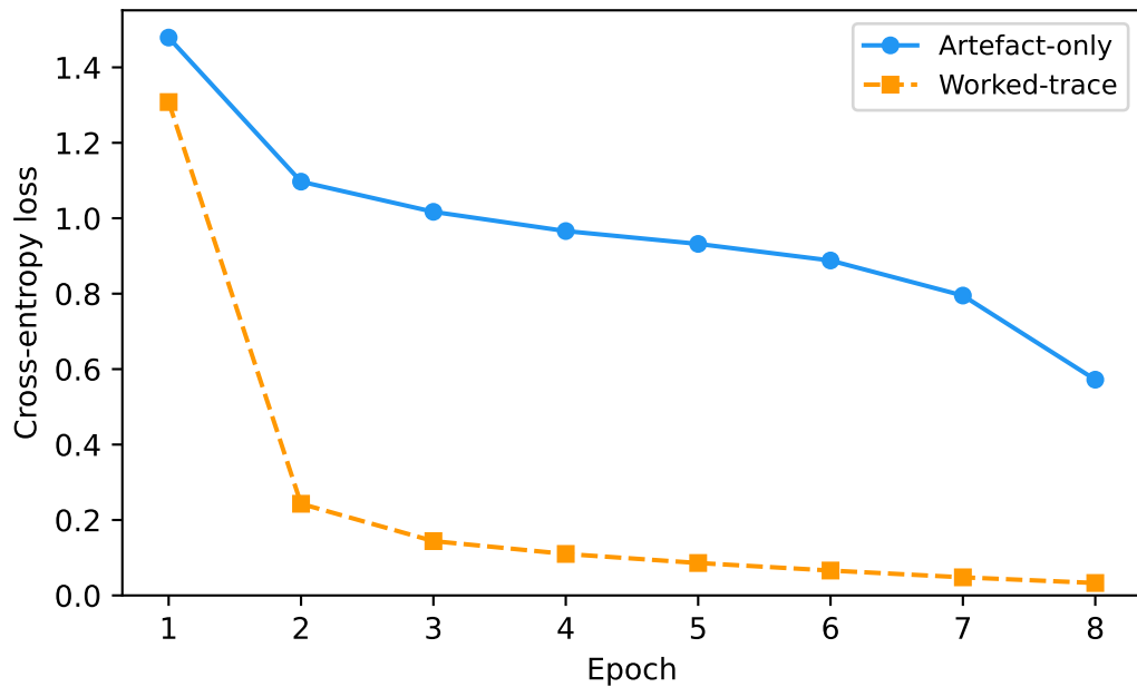
(a) Training loss
