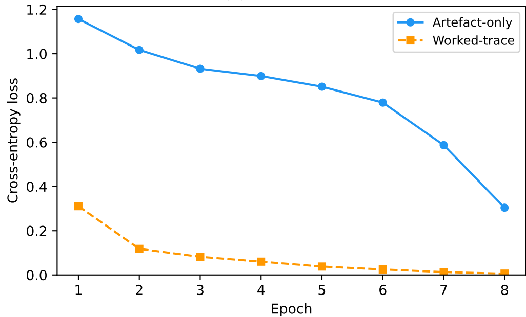
(b) Validation loss
