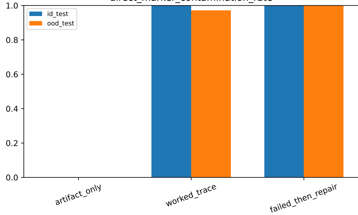
direct_marker_contamination_rate
