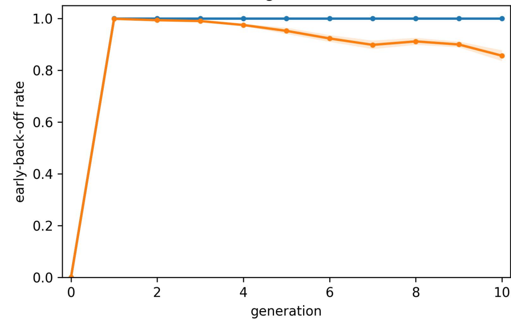
C. Fraction backing off before 100 tokens
