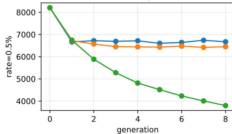
Vocabulary size
