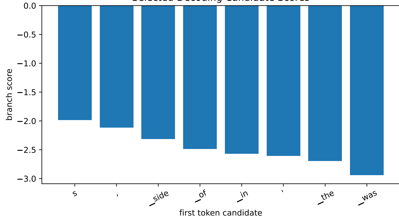
Selected Decoding Candidate Scores
