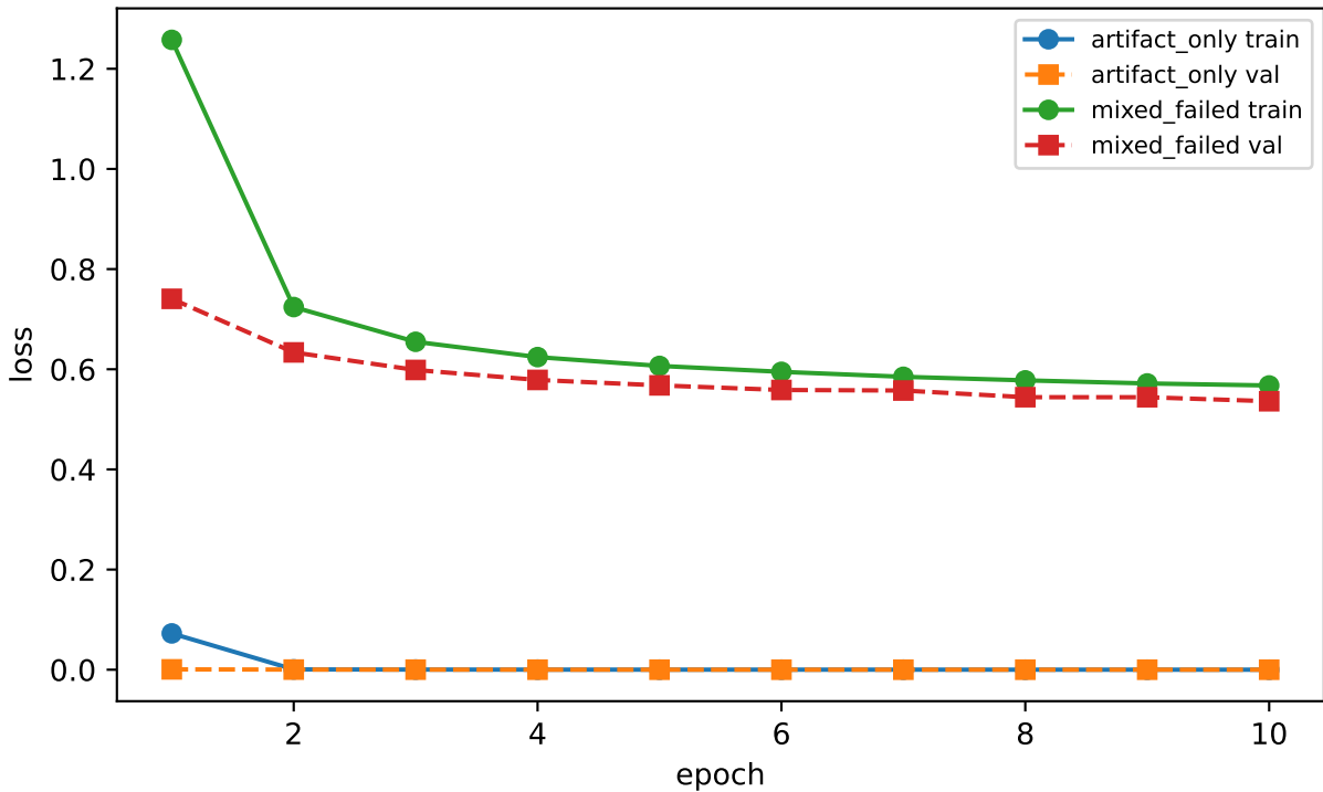
theorem2_positive_tiling_artifact_learning_bridge_mild_ood_ep10 training
