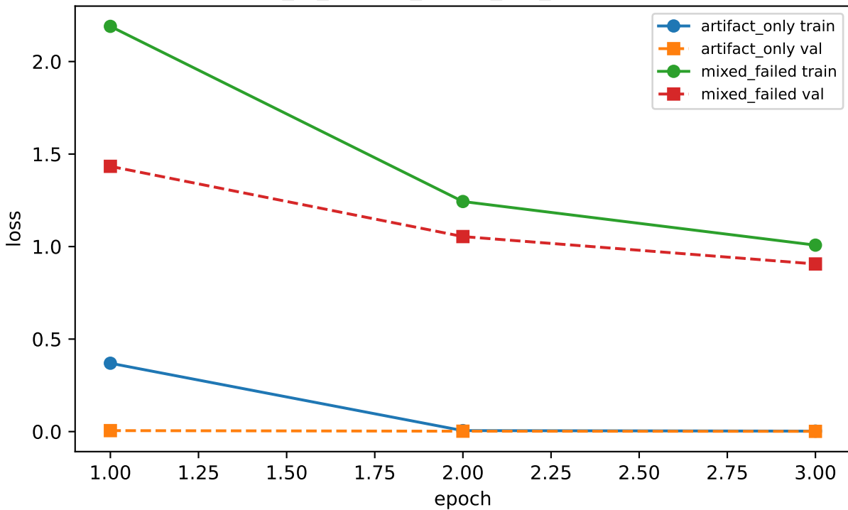
tmp_t2_artifact_sanity_det_ep3 training
