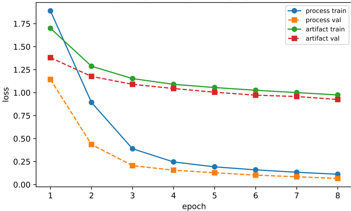
theorem2_taskA_addition_process_vs_artifact training
