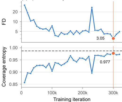
(a) Speaker identity
