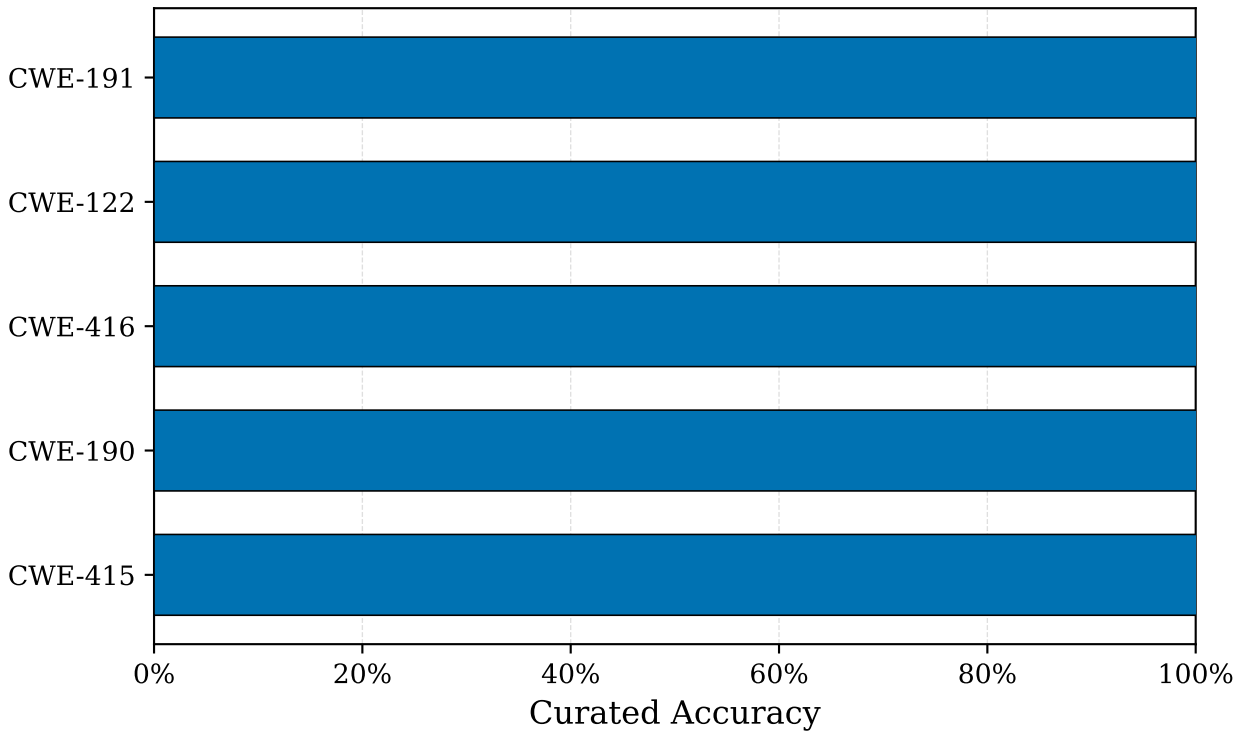
CWE Category
