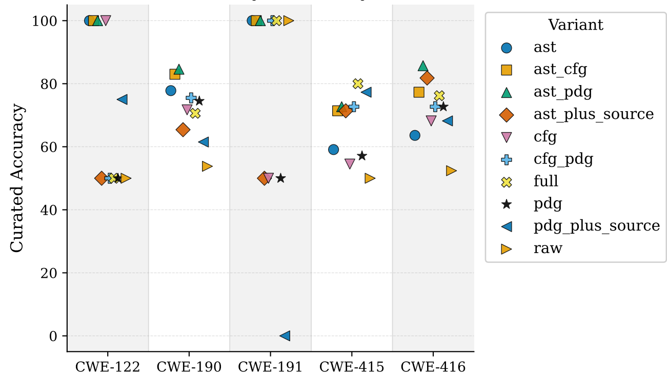
Curated Accuracy vs CWE: by Variant
