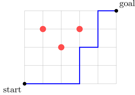
Figure 1: A grid with m = 5 columns and n = 4 rows. The three red points are blocked; the blue line is one of the admissible paths.
