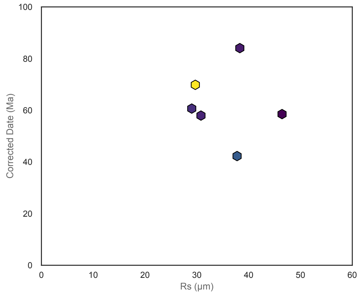
Sample AN01 - AHe
