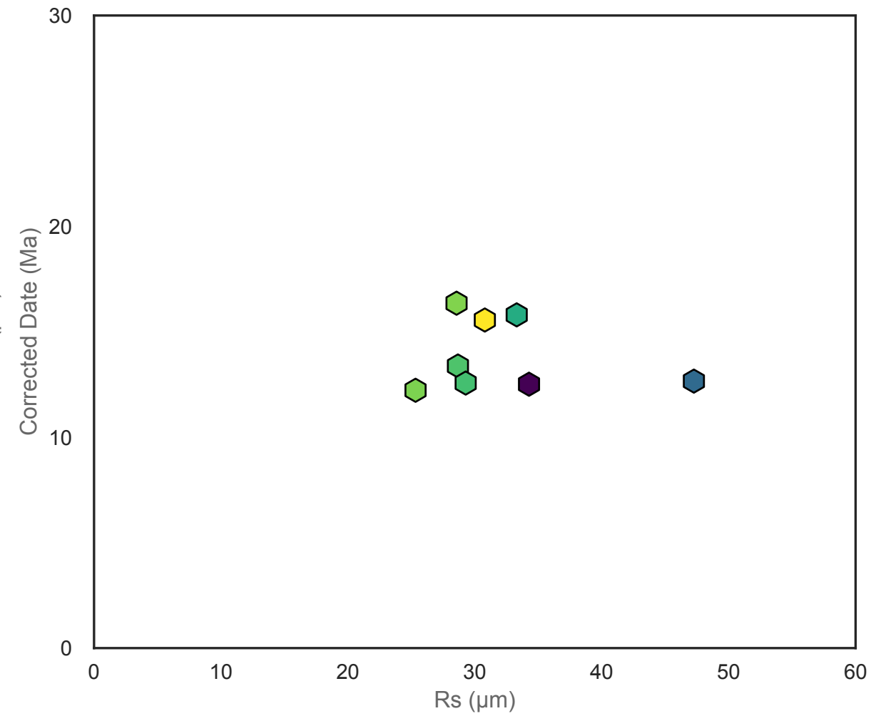
Sample AN03 - AHe
