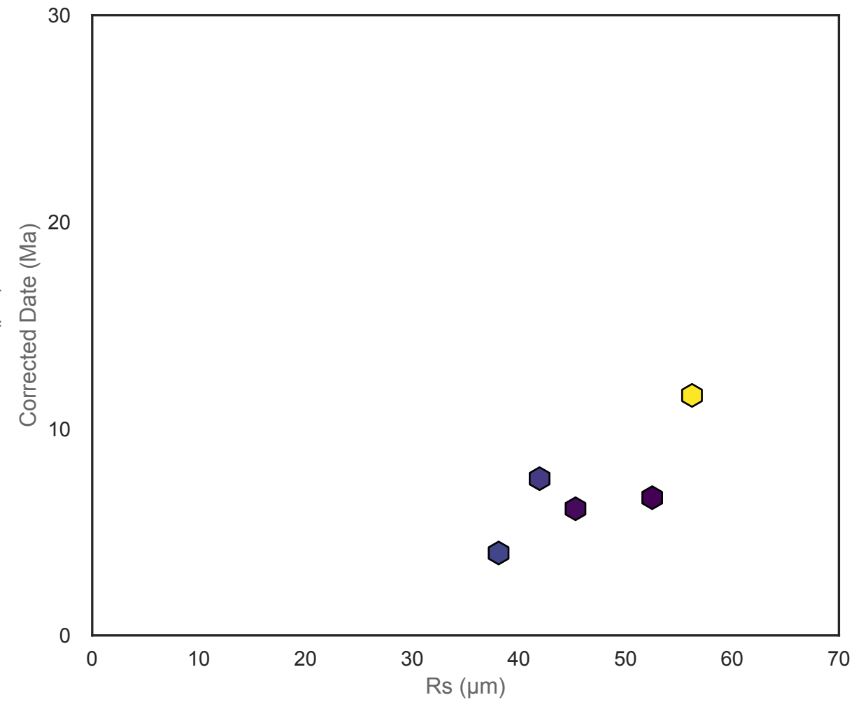
Sample AN04 - AHe
